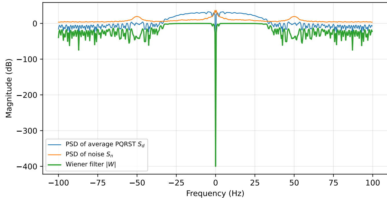
PSD of desired signal, noise, and Wiener filter
